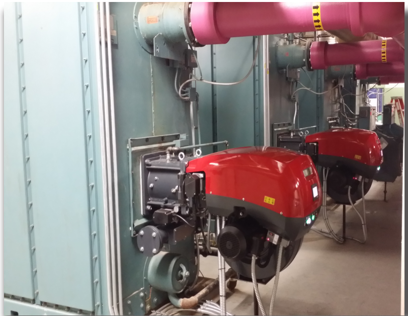
(2) Riello RS 500 Burners
